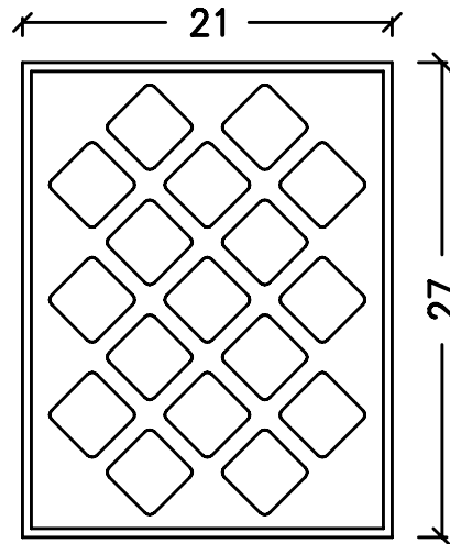
17 Lites 21" x 27"
